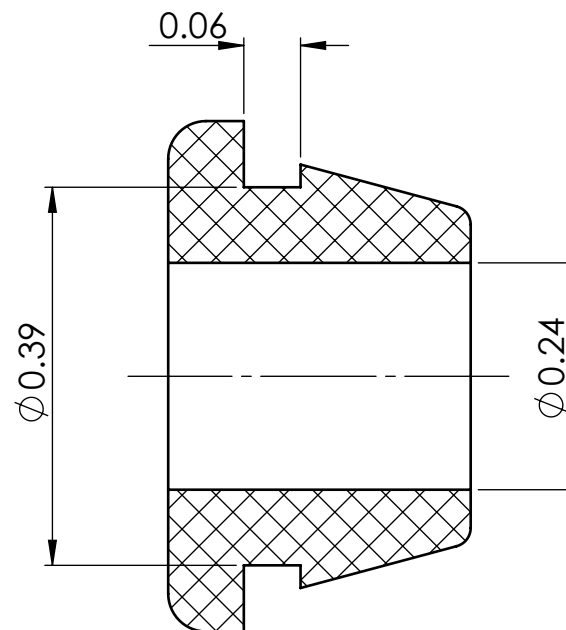
SECTION Y-Y
