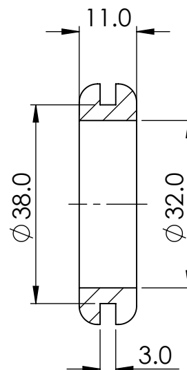
SECTION Y-Y
