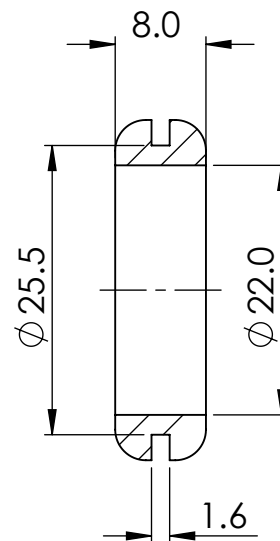
SECTION Y-Y
