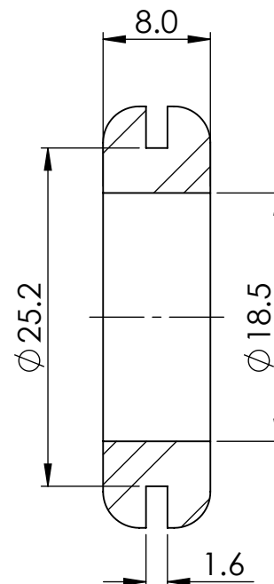
SECTION Y-Y
