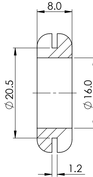
SECTION Y-Y
