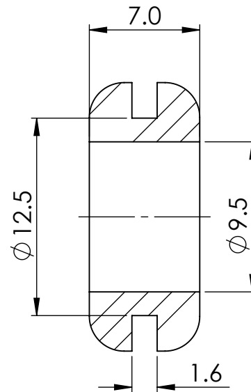
SECTION Y-Y
