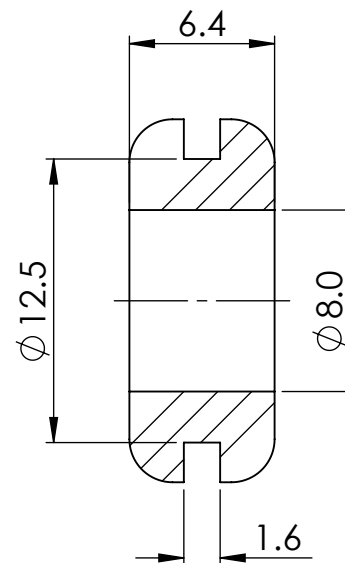
SECTION Y-Y
