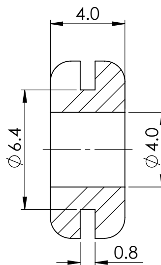
SECTION Y-Y
