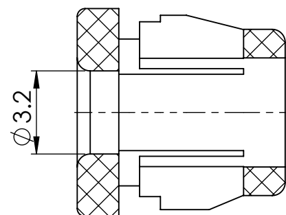
SECTION Y-Y
