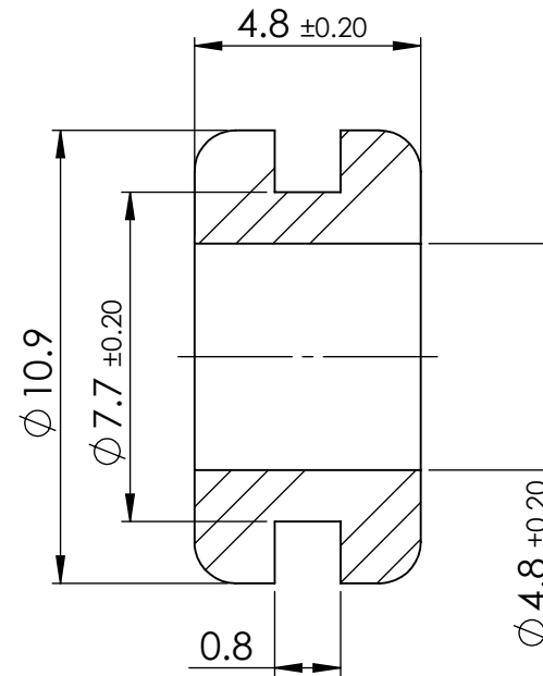
SECTION Y-Y
