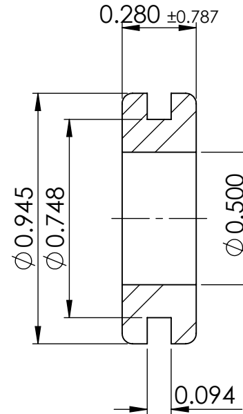
SECTION Y-Y
