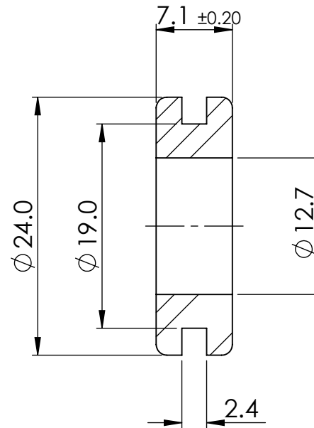
SECTION Y-Y
