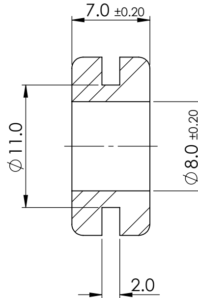
SECTION Y-Y SCALE 3 : 1
