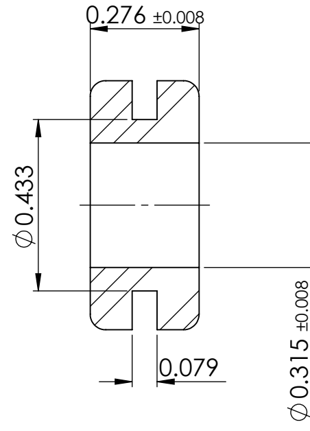
SECTION Y-Y SCALE 3 : 1
