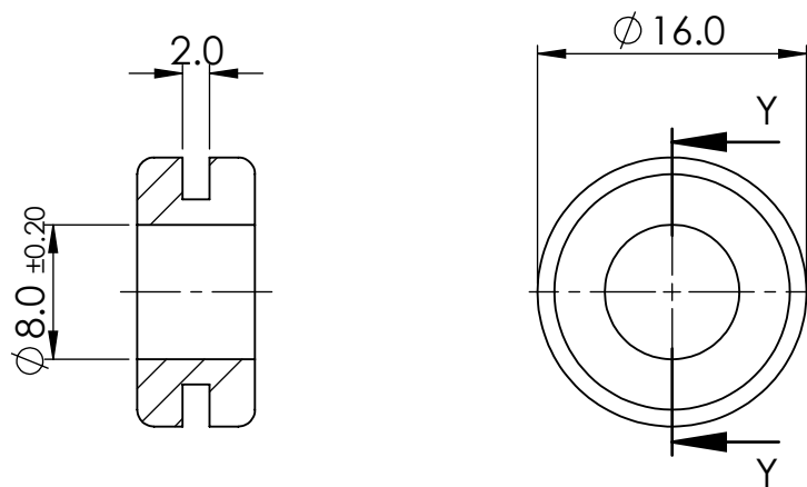
SECTION Y-Y SCALE 2 : 1
