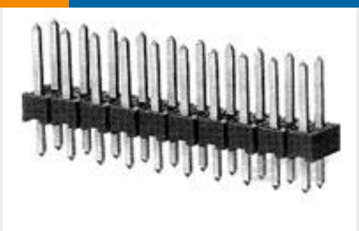
TE Model / Part #826632-7 7P AMPMODU II PIN HDR.
